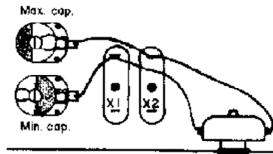
Figure L - Setting crystal trimmers
