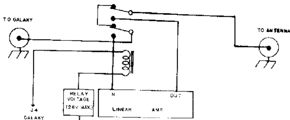
Fig. D. Relay system for use with Linear Amplifier
